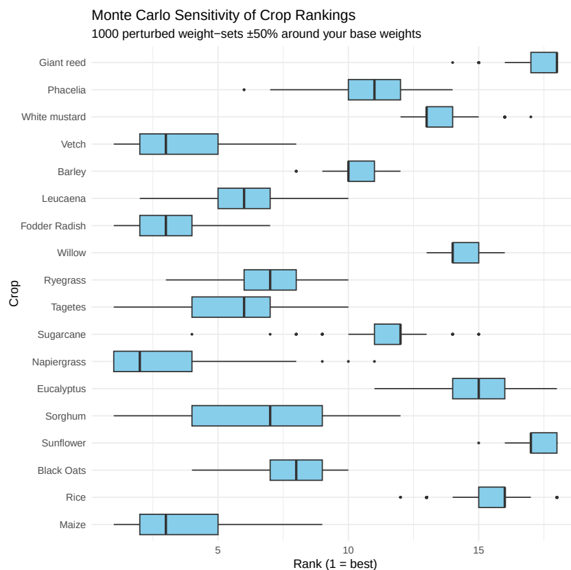
Figure 4: Monte Carlo output
