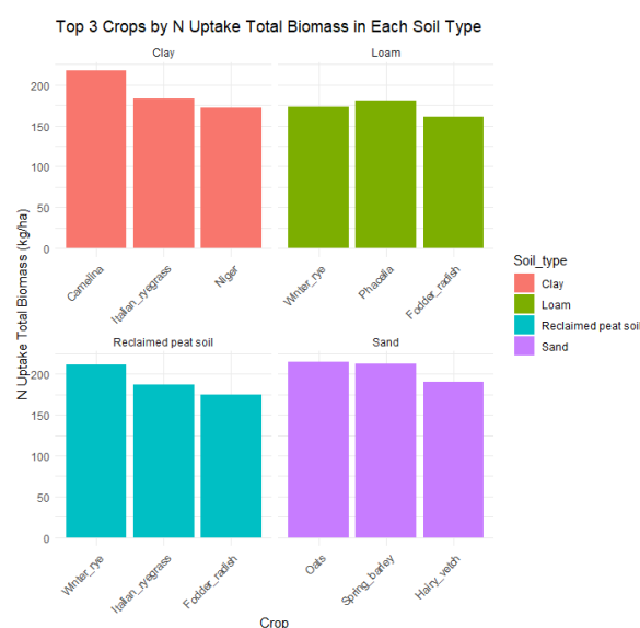
Figure 6: Top N uptake producers by soil type
