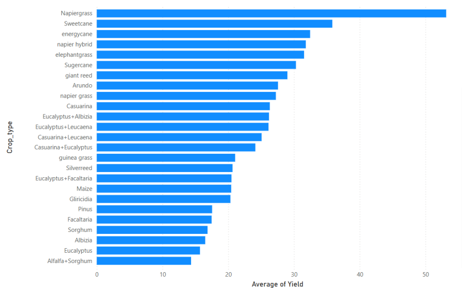
Figure 7: Top biomass producers
