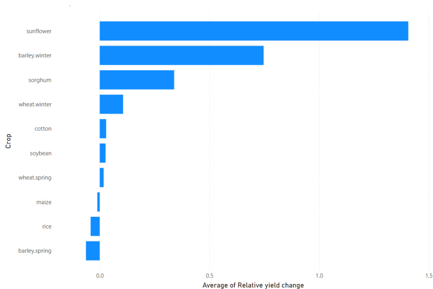
Figure 8: Top no-tillage systems crop
