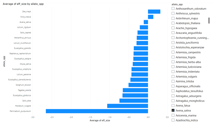
Figure 3: Average Allelopathic strength of selected shortlist crops
