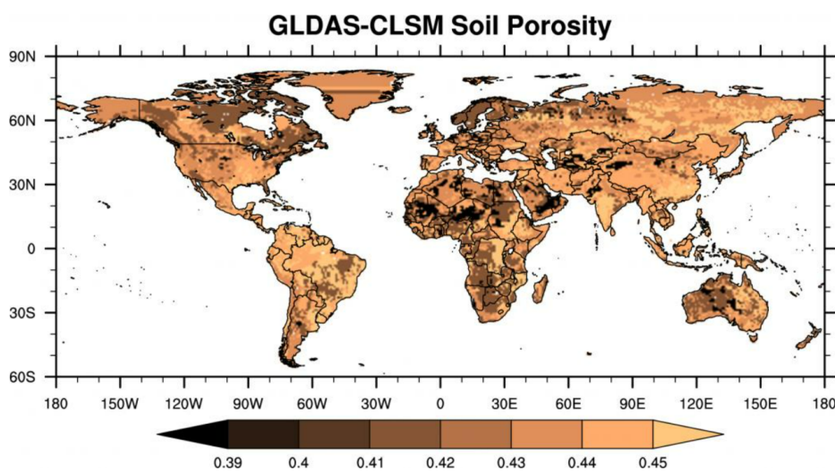
Figure 1: Global Soil Porosity
