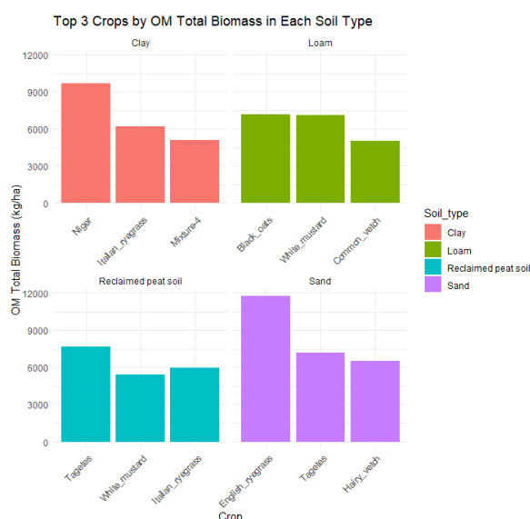
Figure 5: Top organic matter producers by soil type
