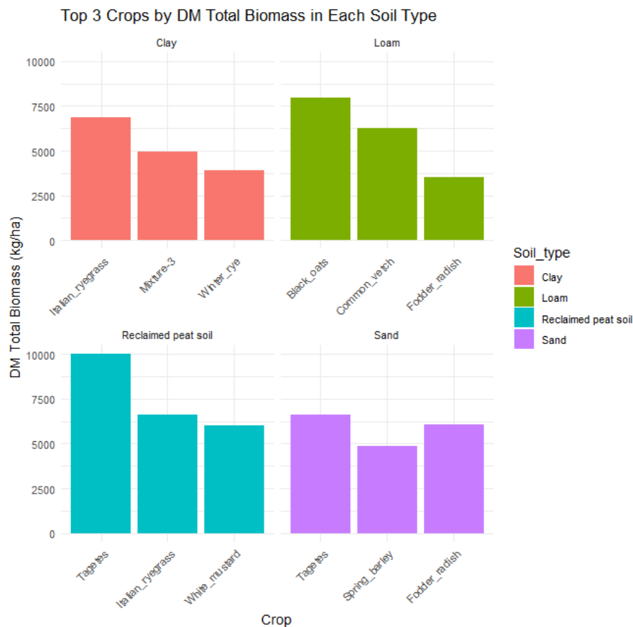
Figure 2: Top Organic Matter Producing Crops by Soil Type
